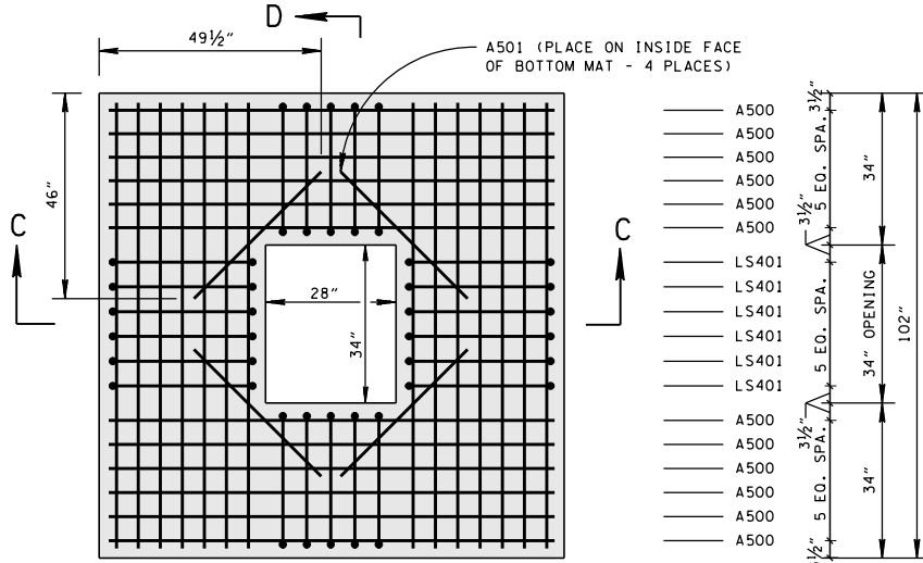
PLAN VIEW
